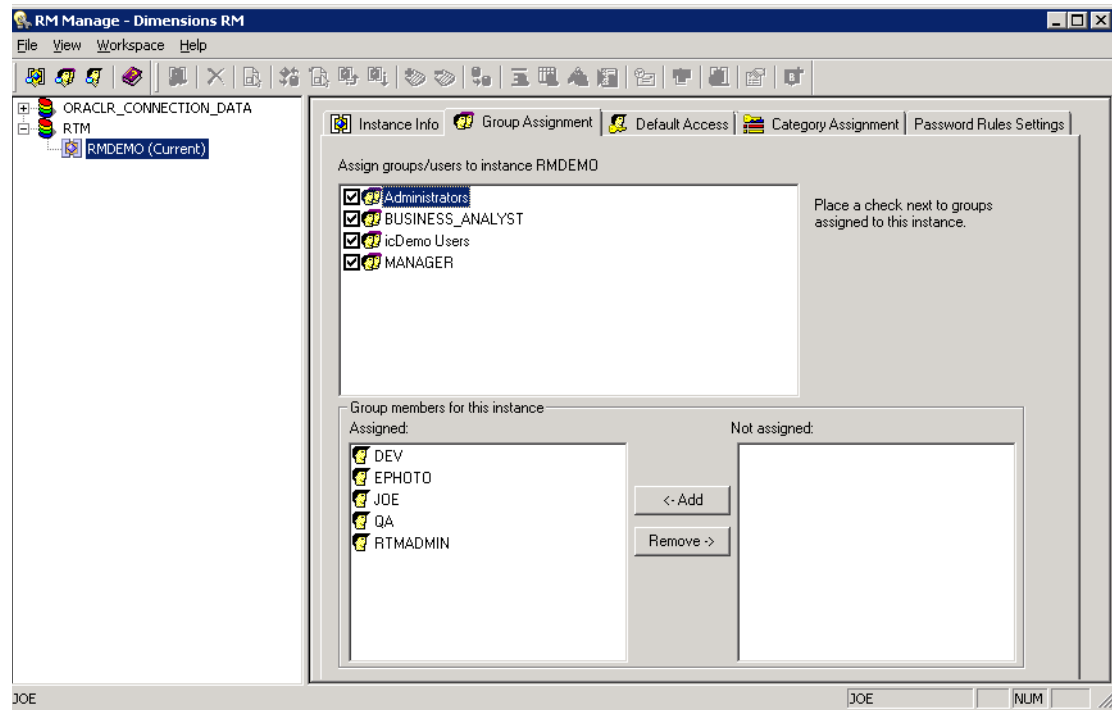
Figure 1-3. RM Manage
