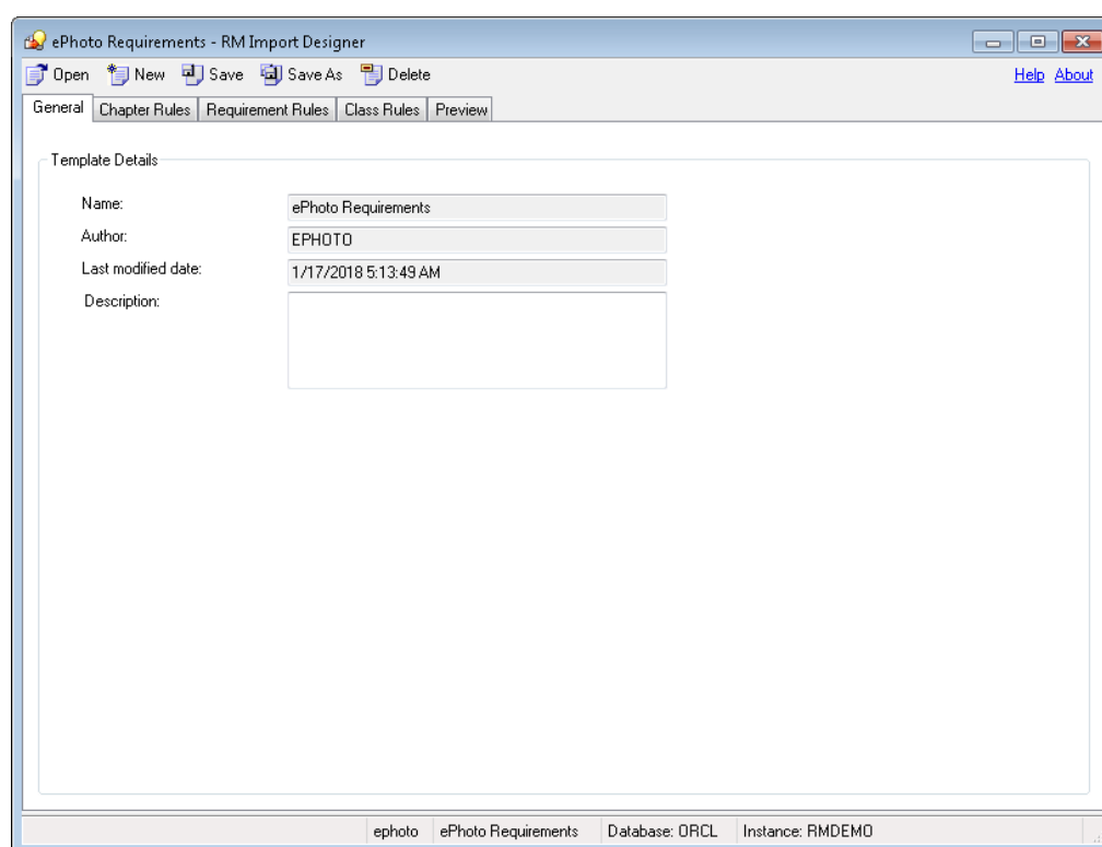
Figure 11-4. General Tab
