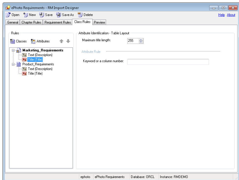
Figure 11-14. Class Rules Tab—Table Option—Alphanumeric Attributes
