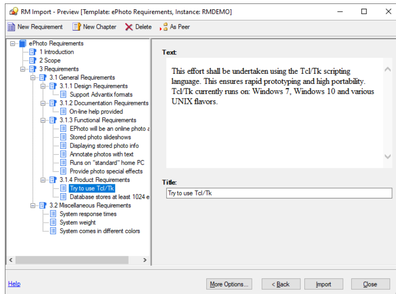
Figure 11-4. Preview Dialog
