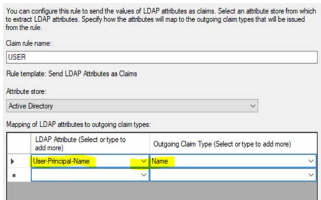
Figure 4-4. Sample Rule
