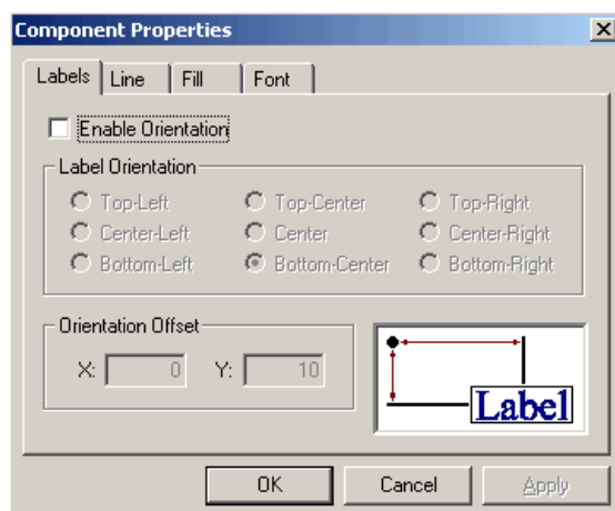
Figure 9-18. Component Properties
