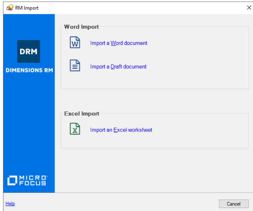
Figure 1-2. RM Import
