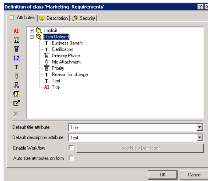
Figure 9-17. Class Definition
