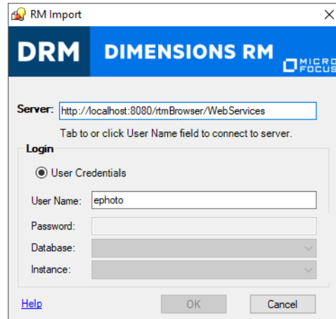
Figure 11-1. Login Dialog
